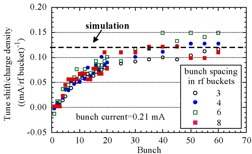
Measurements of vertical tune shift as a function of bunch number in a bunch train in KEKB. H. Fukuma, Proceedings of ELOUD02.
