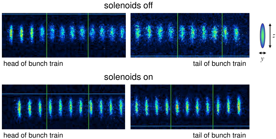
Observations of beam-size increase in KEKB. H. Fukuma, Proceedings of ELOUD04.
