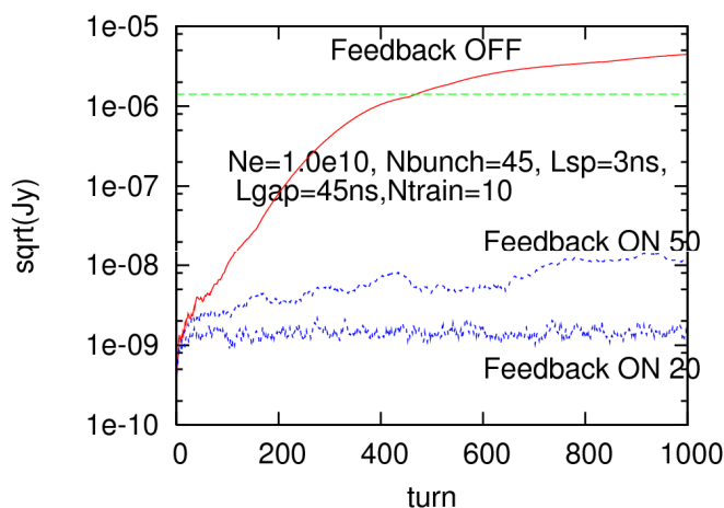
Simulation of fast ion instability in a recent 6.7 km lattice for the ILC damping rings, by Kazuhito Ohmi.
