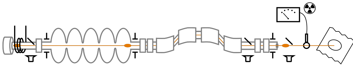
Figure 5: Sketch of multiple types of diagnostic tools along the linac and dosimetric measurement outside.
